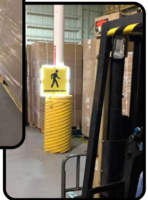
3 Forklift operator is alerted to the presence of a pedestrian by flashing sign.
