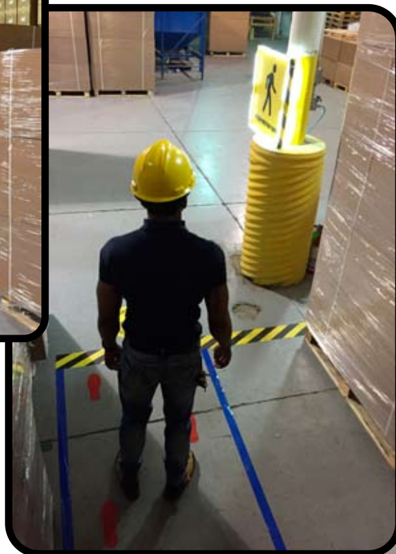
2 Pedestrian entering forklift lane activates motion sensor to start sign blinking.
